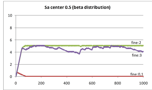
Fig. 20. Fine evolution for BCT (d) and BestPathMinimax , with a uniform distribution of risk tolerance and a beta distribution of social awareness centered at 0.5
