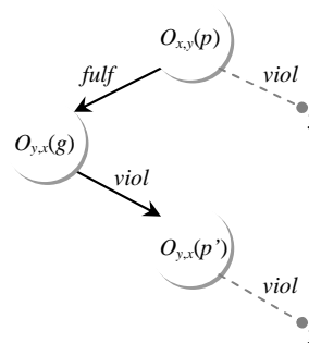
Fig. 1. Sample commitment tree
