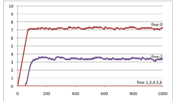
Fig. 11. Fine evolution for BCT (e) and DoubleFulfillmentBalance
