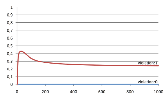
Fig. 6. Violation cumulative average (%) for BCT (c) and LocalTD
