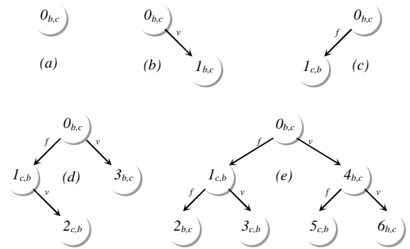
Fig. 4. Binary commitment trees 2 : each node Id_{i,j} is an obligation, where i is the bearer and j is the counterparty
