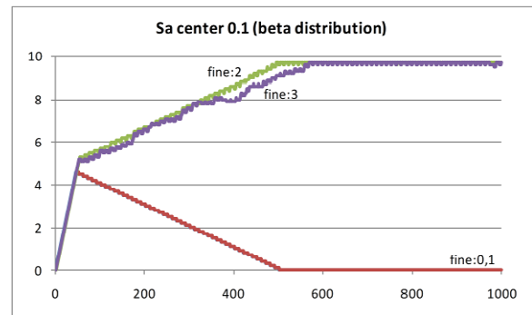
Fig. 21. Fine evolution for BCT (d) and BestPathMinimax , with a uniform distribution of risk tolerance and a beta distribution of social awareness centered at 0.1
