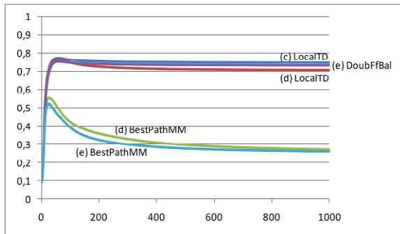
Fig. 15. Contract cumulative average (%) for the five settings
