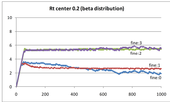
Fig. 18. Fine evolution for BCT (d) and BestPathMinimax , with a beta distribution of risk tolerance centered at 0.2 and a uniform distribution of social awareness
