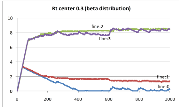
Fig. 17. Fine evolution for BCT (d) and BestPathMinimax , with a beta distribution of risk tolerance centered at 0.3 and a uniform distribution of social awareness
