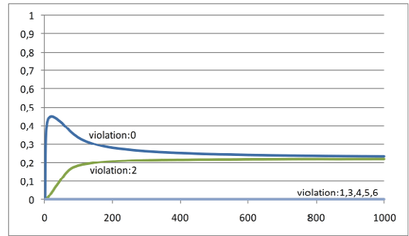
Fig. 12. Violation cumulative average (%) for BCT (e) and DoubleFulfillmentBalance
