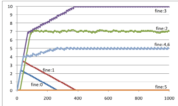
Fig. 13. Fine evolution for BCT (e) and BestPathMinimax
