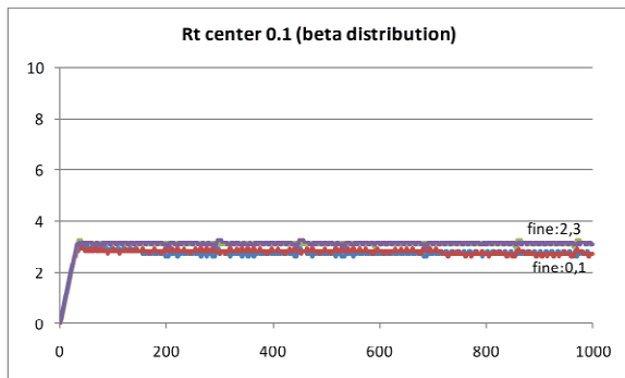
Fig. 19. Fine evolution for BCT (d) and BestPathMinimax , with a beta distribution of risk tolerance centered at 0.1 and a uniform distribution of social awareness
