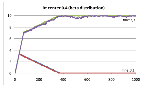
Fig. 16. Fine evolution for BCT (d) and BestPathMinimax , with a beta distribution of risk tolerance centered at 0.4 and a uniform distribution of social awareness
