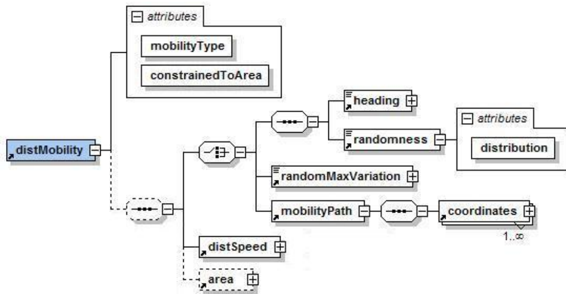
Figure 4.22: Disturbance Mobility
