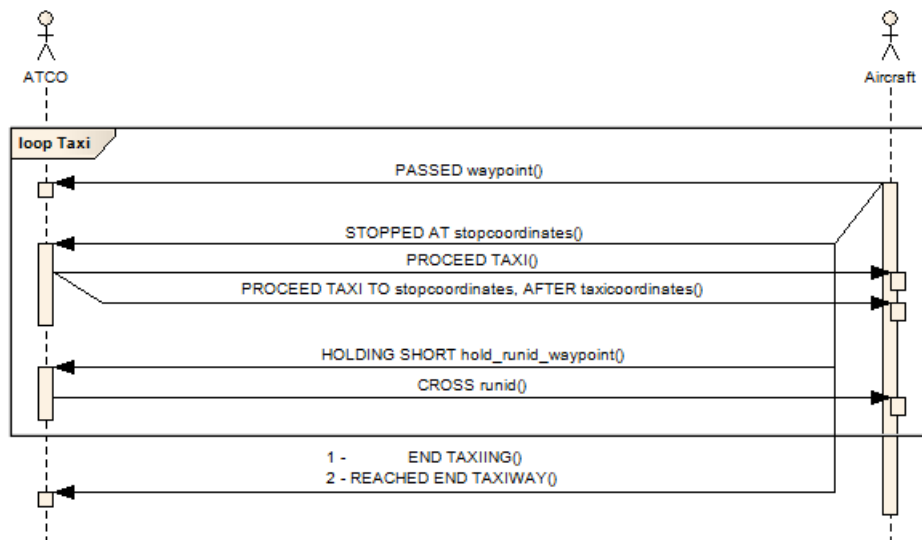
Figure 6.4: Taxi Protocol
