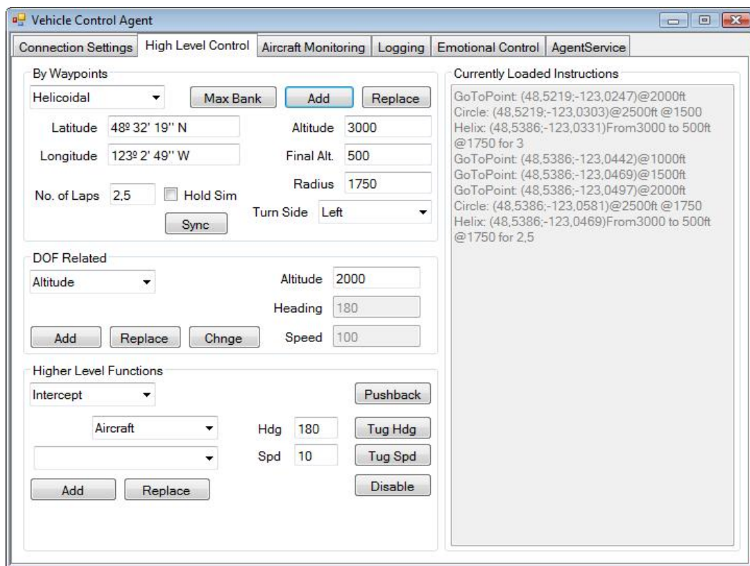
Figure 6.11: Vehicle Control Agent Interface
