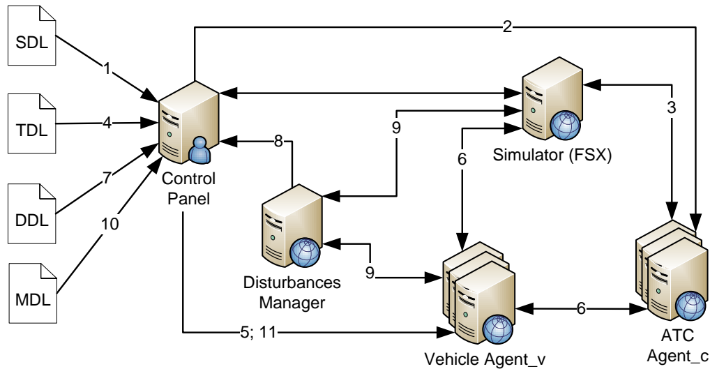
Figure 3.10: Simplified Data Flow Model
