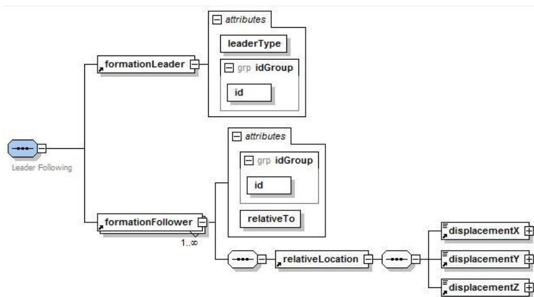
Figure 4.29: Formation Specification with Leader and Followers
