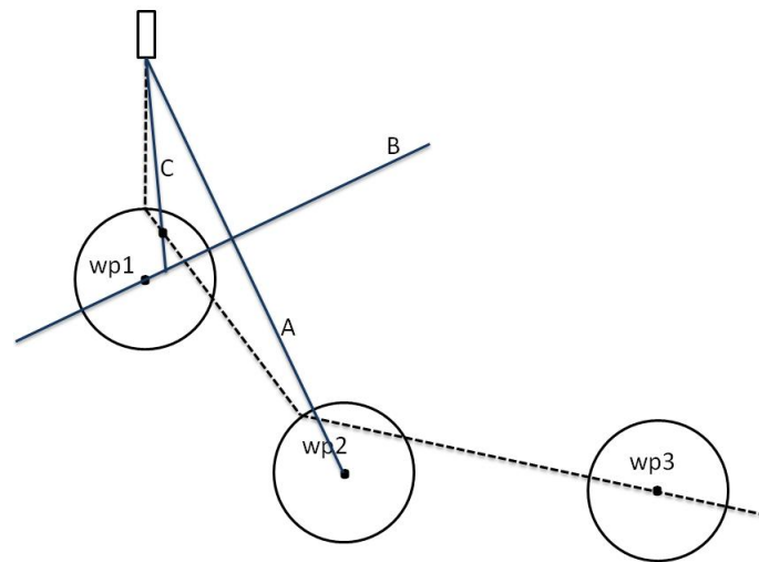
Figure 6.19: Waypoint Approach Submarine Navigation
