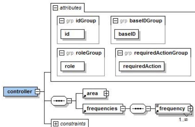
Figure 4.16: Controller Element Definition
