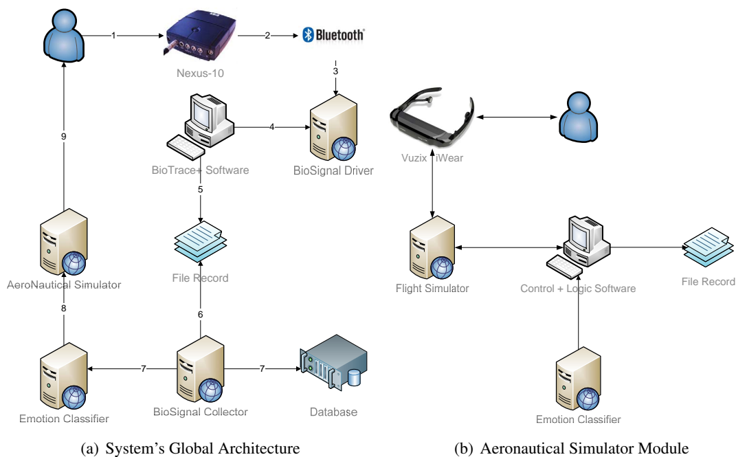
Figure 5.3: System Global Architecture (a) and Aeronautical Simulator Module (b)
