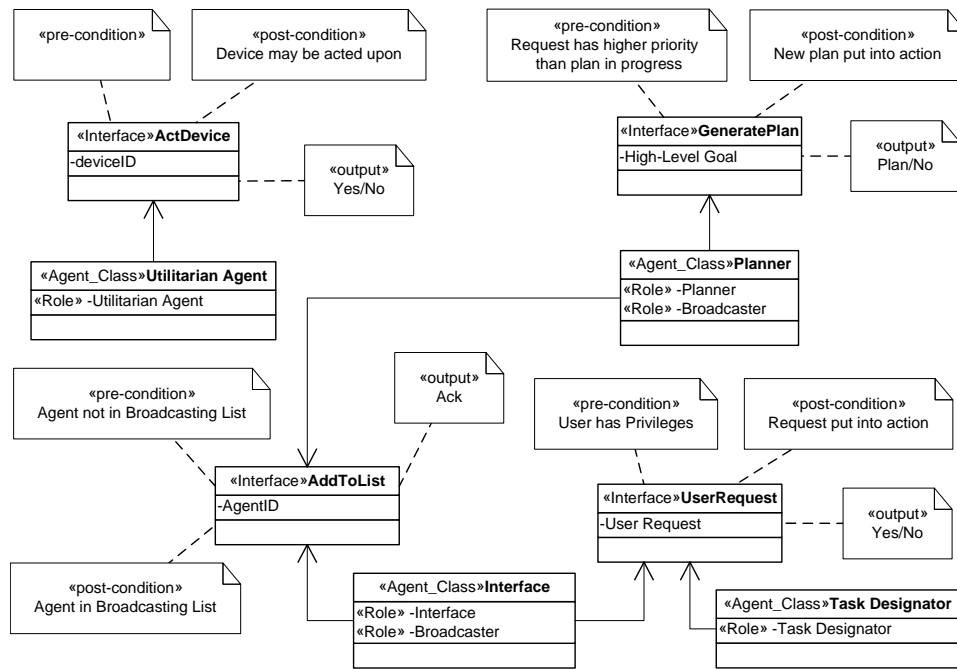
Figure 3.8: Service Model
