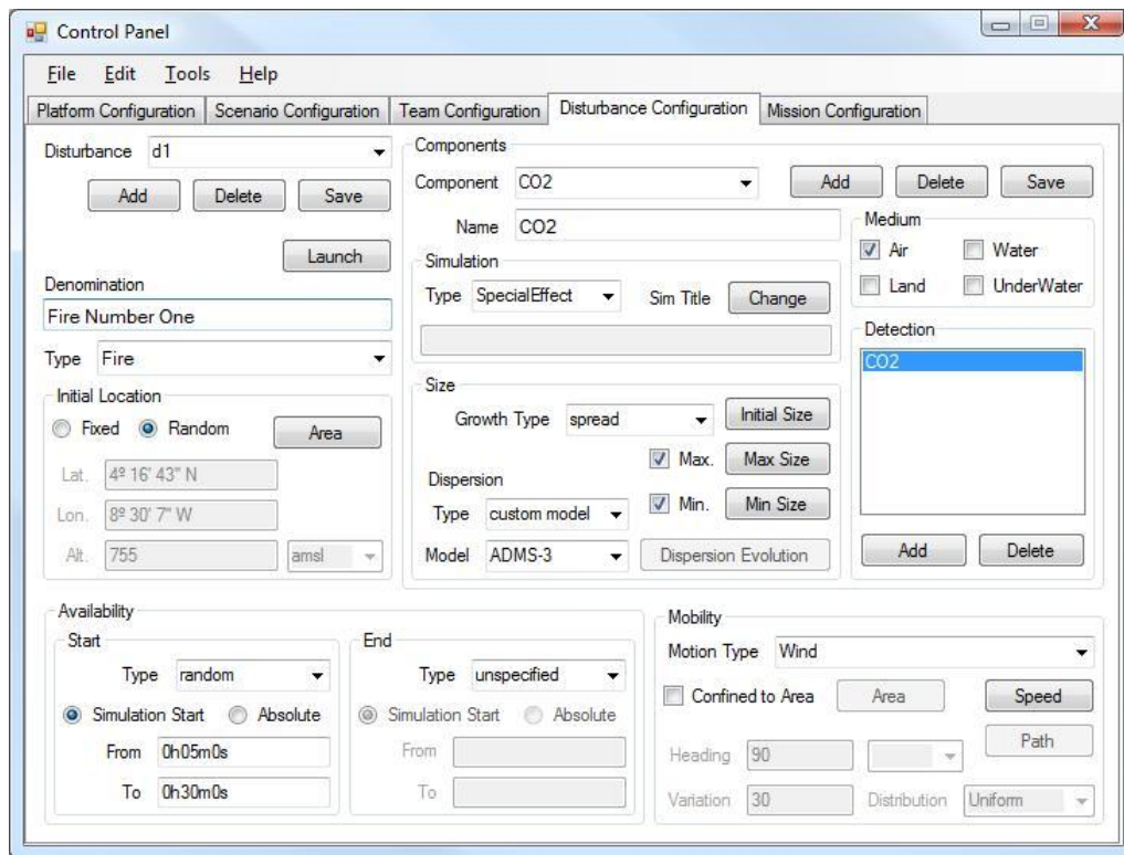
Figure 5.15: Control Panel – Disturbances Configuration
