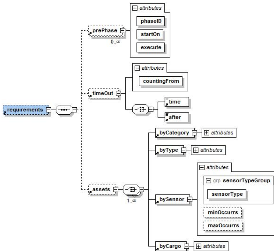
Figure 4.27: Phase Requirements
