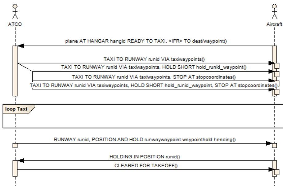
Figure 6.5: Takeoff Protocol
