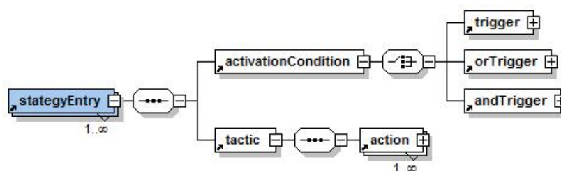
Figure 4.32: Strategy Entry
