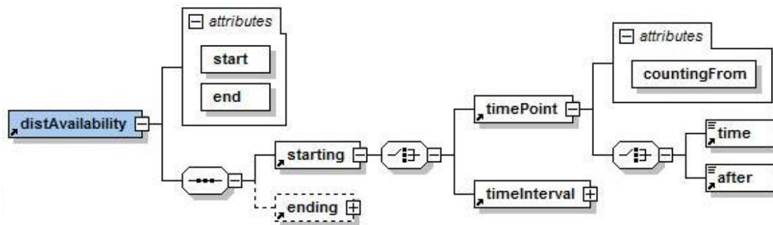
Figure 4.21: Disturbance Availability
