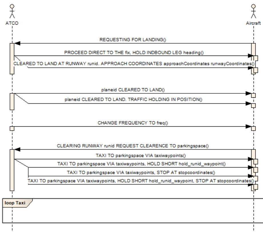
Figure 6.6: Land Protocol
