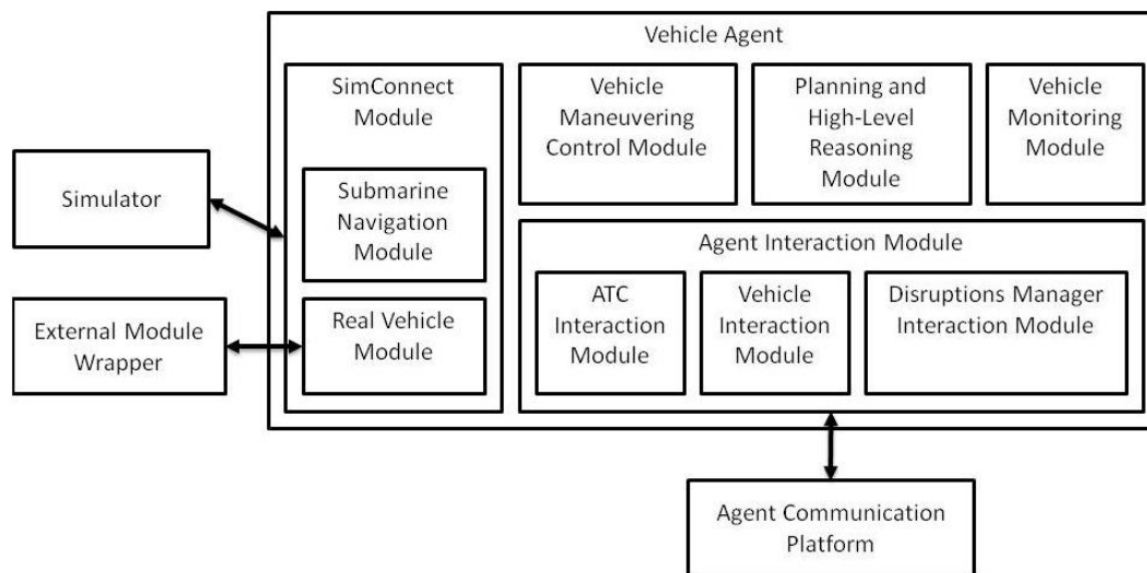
Figure 6.10: Vehicle Agent Internal Architecture
