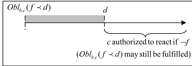
Figure 6.1: Directed obligation with deadline.
