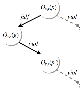
Figure 8.1: Sample commitment tree.
