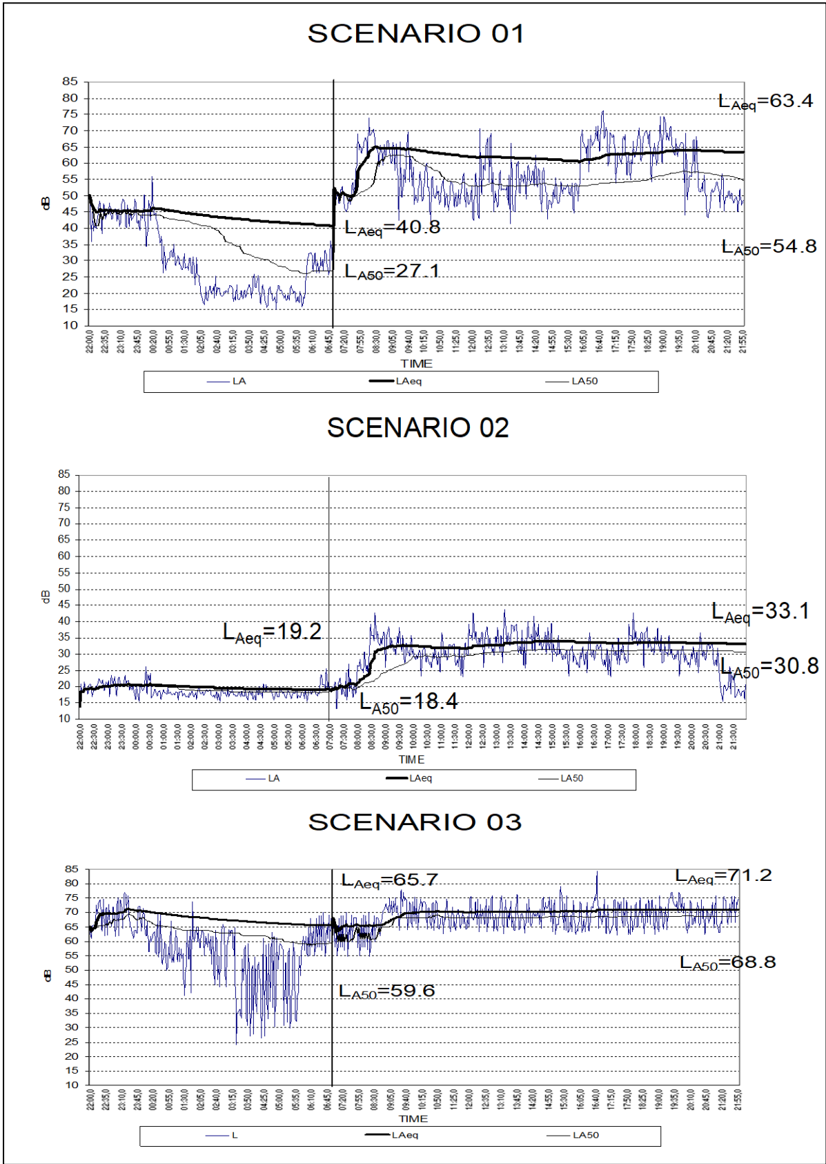
Fig. 1: Three acoustic scenarios.
