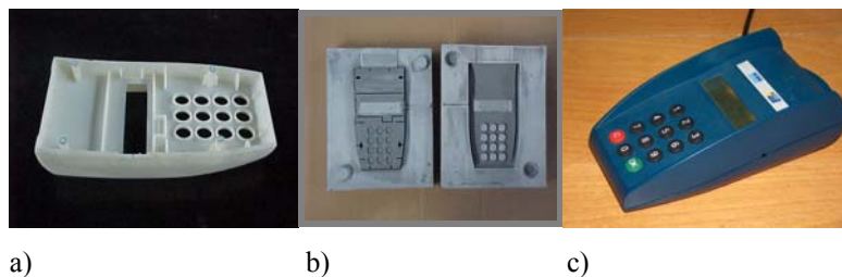
Fig. 1 - New products development using composite moulds: a) ABS prototype model obtained by High Speed Machining (HSM) and used as a master to produce the composite mould; b) composite mould in aluminium filled resin; c) final component with the thermoplastic injected part.
