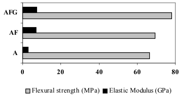
Fig. 9 - Flexural strength and elastic modulus of the A, AF and AFG materials.
