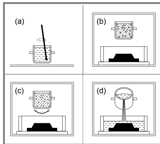
Fig.4 - Processing method using vacuum pouring: a) manual component mixture; b) first degassing; c) second degassing with agitation; d) vacuum pouring.
