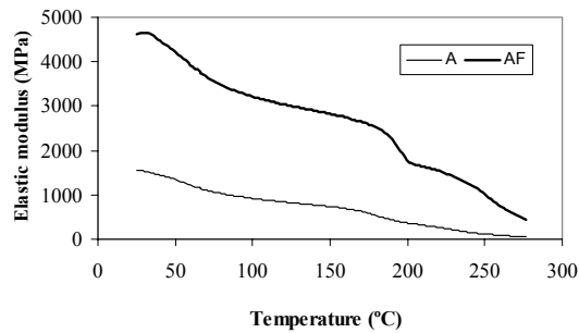
Fig. 10 - Elastic modulus as a function of temperature for the neat resin A and aluminium filled epoxy AF, obtained in DMTA tests.
