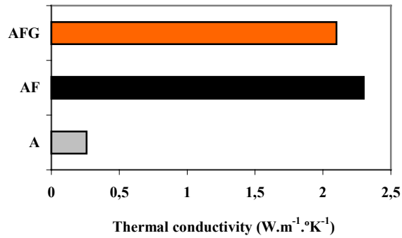
Fig. 12 - Thermal conductivity of the three tested materials (Kirksite alloy Z35541 – ASTM B86 [14] has 105.0 W.m -1 .°K -1 ).
