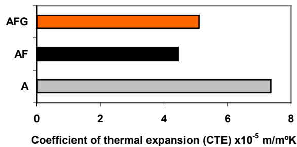
Fig. 11 - CTE of A epoxy resin and of the two composites; AF and AFG.
