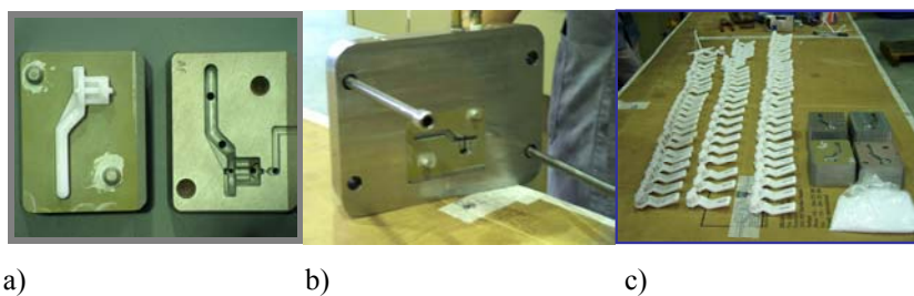
Fig. 2 - Epoxy based composite mould for thermoplastic injection of a latch: a) composite mould; b) preparation of the core and cavity in the standard plate of an industrial injection machine; c) pre series of the latch.
