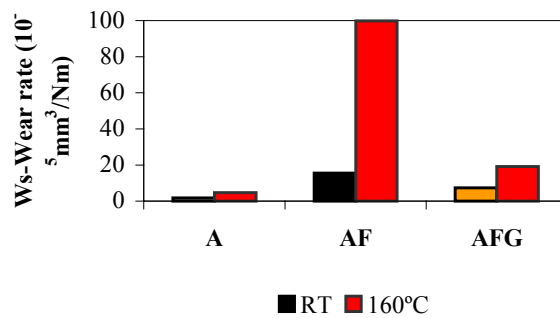
Fig. 13 - Specific wear rate of epoxy (A), epoxy with aluminium (AF) and epoxy with aluminium and fibres (AFG) systems, at room temperature and at 160°C, determined in the reciprocating tribometer.
