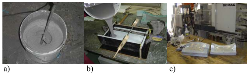
Fig. 7 - Back up of the first half mould: a) mixing of the resin with the catalyst and the aluminium metallic particles; b) casting the slurry over the metallic shell; c) final mould.
