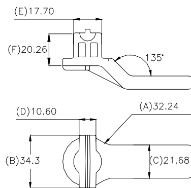
Fig. 14 - Latch model dimensions used in the geometric control.
