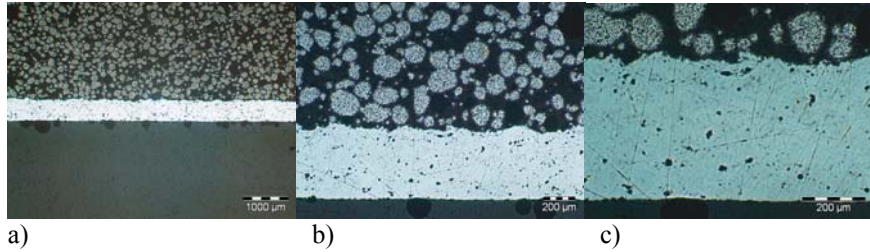
a) b) c) Fig. 8 - Cross-section of one mould composed by a metallic layer and a back up in composite resin; a) cross section of the mould; b) detail of the two phases; c) detail of the metallic shell, showing small round black dots, corresponding to the shell porosity.
