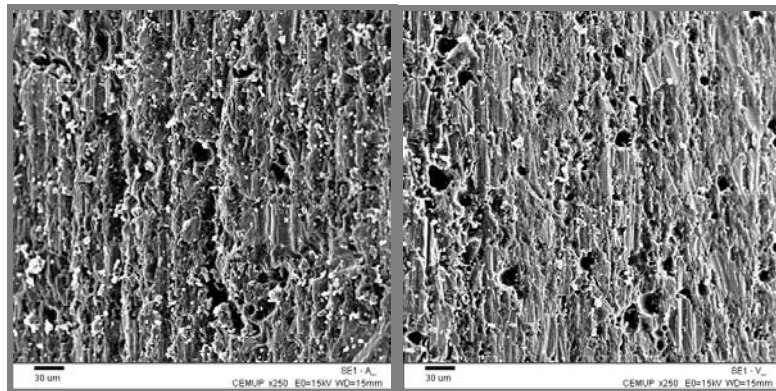
Fig. 15 - SEM images of the moulding cavity surfaces, revealing the degree of excoriation occurred in the thermoplastic flow direction of the: a) AF mould with more severe excoriation, deeper grooves, and; b) AFG moulds, with softer surfaces.
