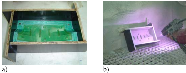
Fig. 5 - Arc spray metal tooling: a) wood box containing the stereolithography RP model coated with the release agent; b) deposition of the metallic coating.
