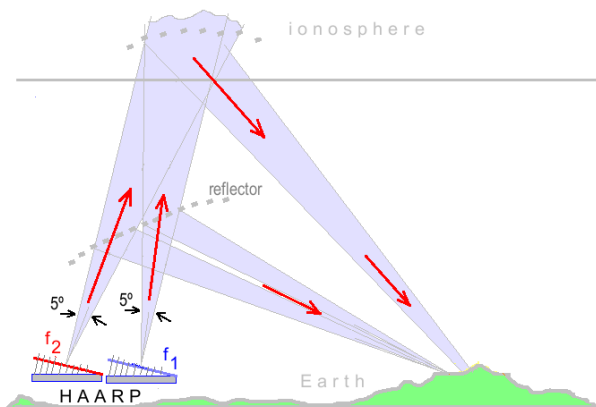
Fig. 10 Aperture of HAARP antennas, and its implications.
