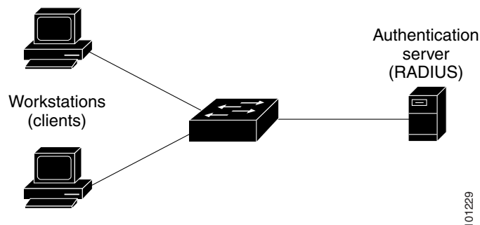
Figure 9-5 Multiple Host Mode Example
