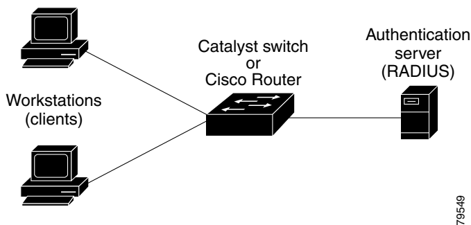
Figure 10-1 Web-Based Authentication Device Roles
