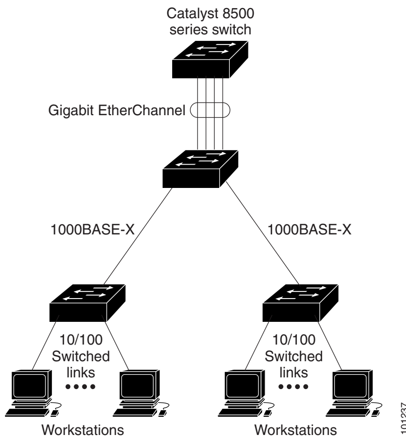
Figure 35-1 Typical EtherChannel Configuration
