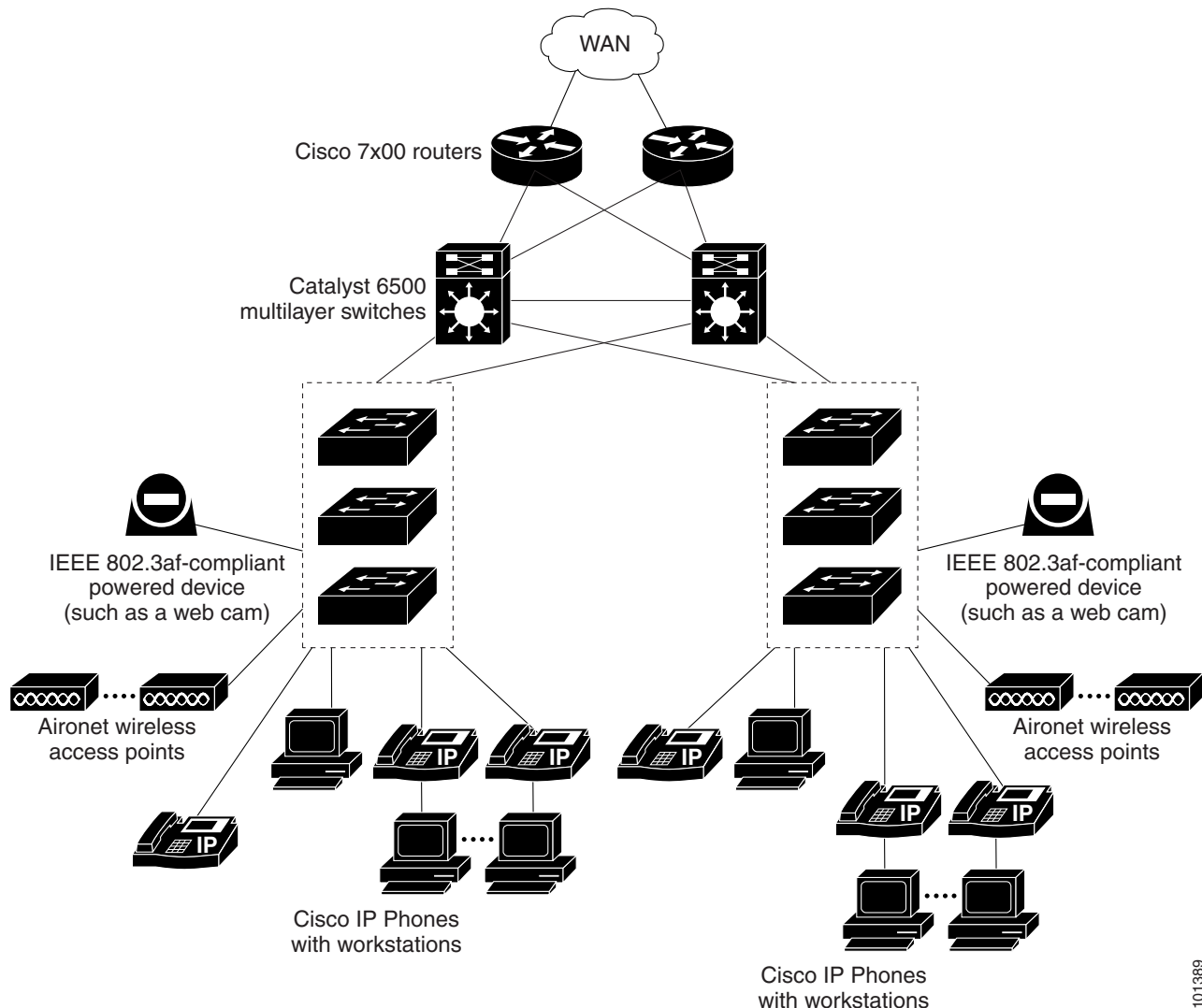
Figure 1-4 Switches in Wiring Closets in a Backbone Configuration
