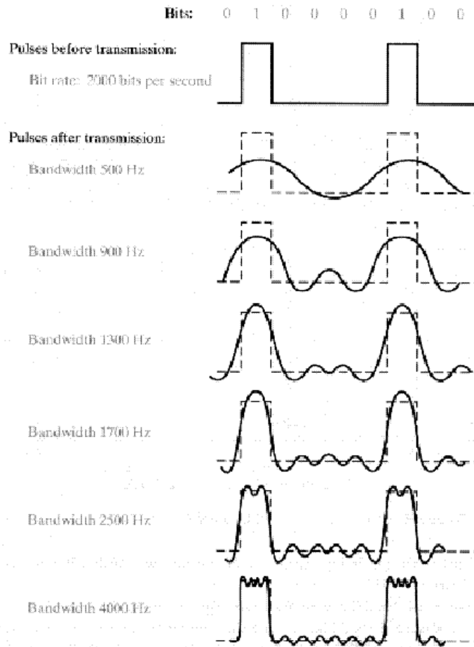
FIGURE 2.9 Effect of bandwidth on a digital signal.
