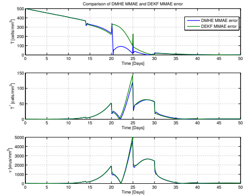
Fig. 4. Comparison between the absolute error of the MMAE using a bank of DMHEs and using a bank of decimated EKFs.
