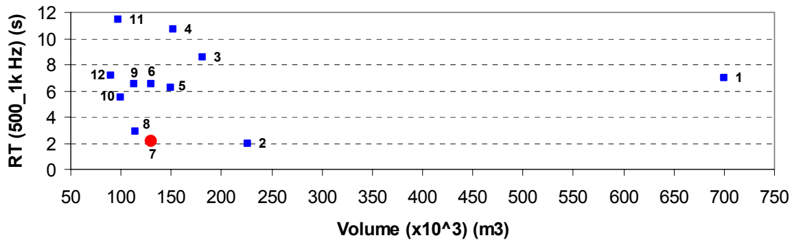
Figure 12 – Average RT (500-1k Hz) for twelve mega-churches (Fátima Holy Trinity: red dot).
