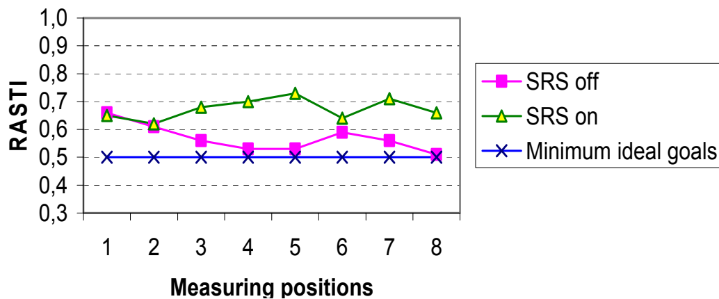
Figure 12 – RASTI values within the church with and without the SRS compared with the minimum ideal goals.
