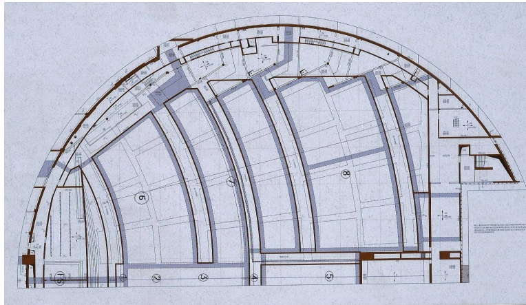
Figure 3 – Holy Trinity church floor half plan with RASTI measuring positions (altar at bottom left).
