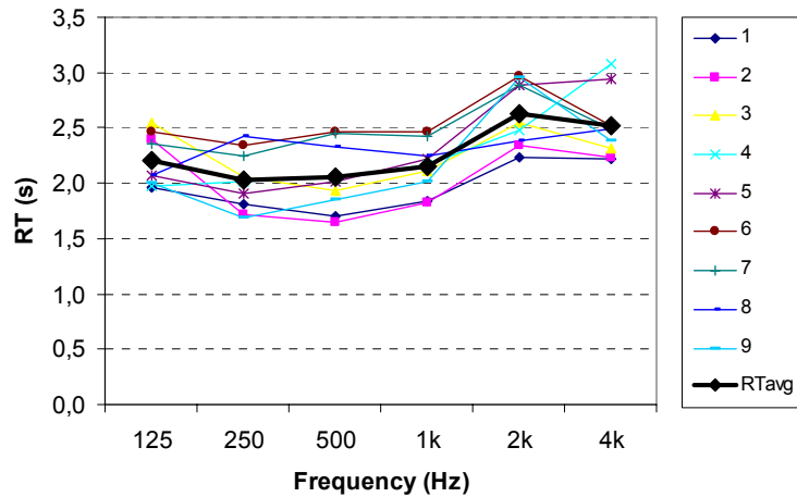
Figure 13 – Spectra of RT values in all the 9 measured points and the RTaverage
