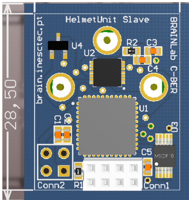
Figure 2: Slave Design (back view)
