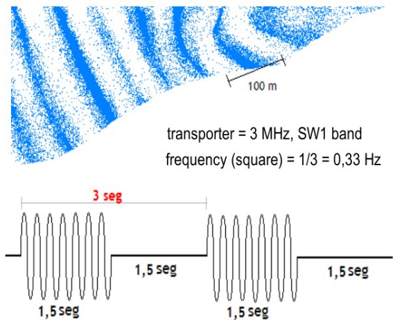
Fig. 8 Some altocumulus ondulatus observed in the town, estimated dimensions and possible frequencies related to them.
