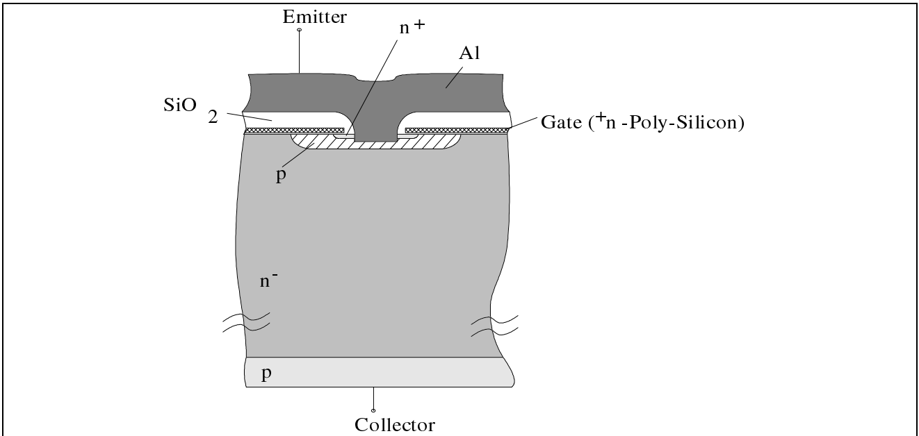
Figure 2 IGBT (Insulated Gate Bipolar Transistor)
