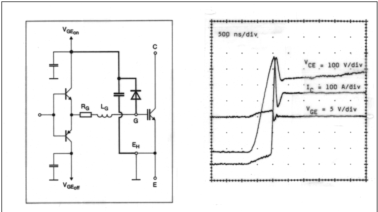
Figure 20 Bias Circuit With Actively Clamped Gate
