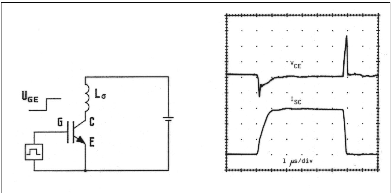
Figure 16 Schematic of Short-circuit I
