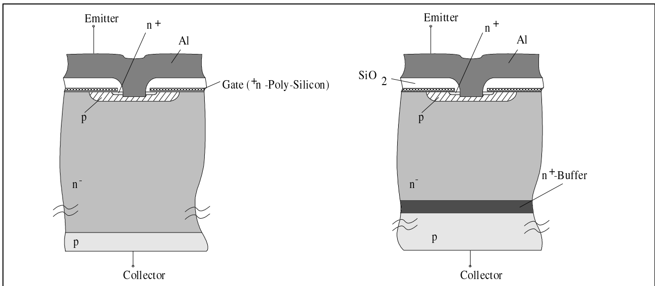
Figure 7 NPT-IGBT (“homogeneous structure”)
