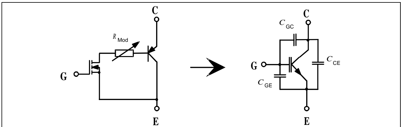
Figure 5 Equivalent Circuit of the IGBT
