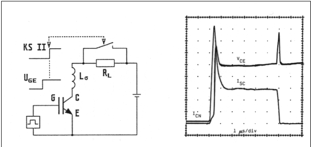
Figure 18 Schematic for Short-circuit Type II
