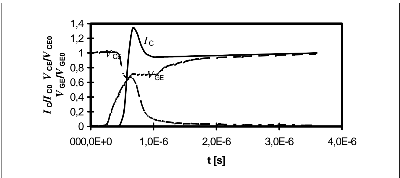
Figure 10 Switch-on with Current Commutating from a Freewheeling Circuit
