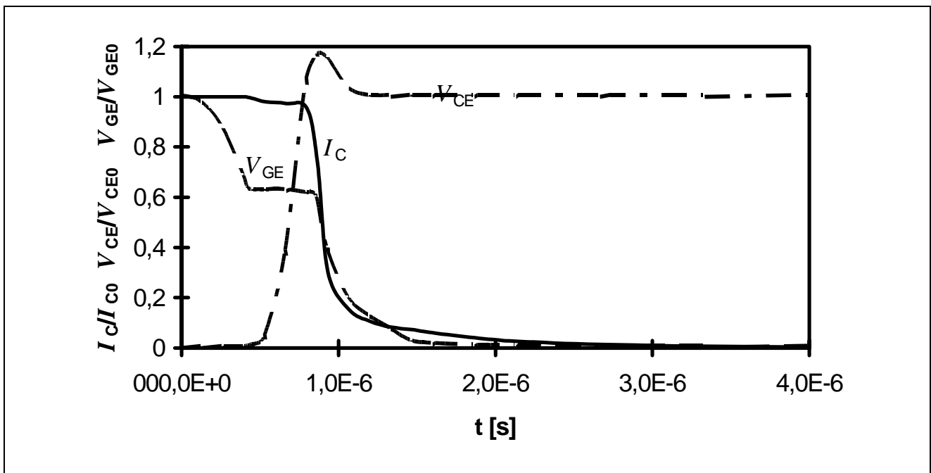
Figure 11 Turn-off of an Inductive Load into a Freewheeling Circuit
