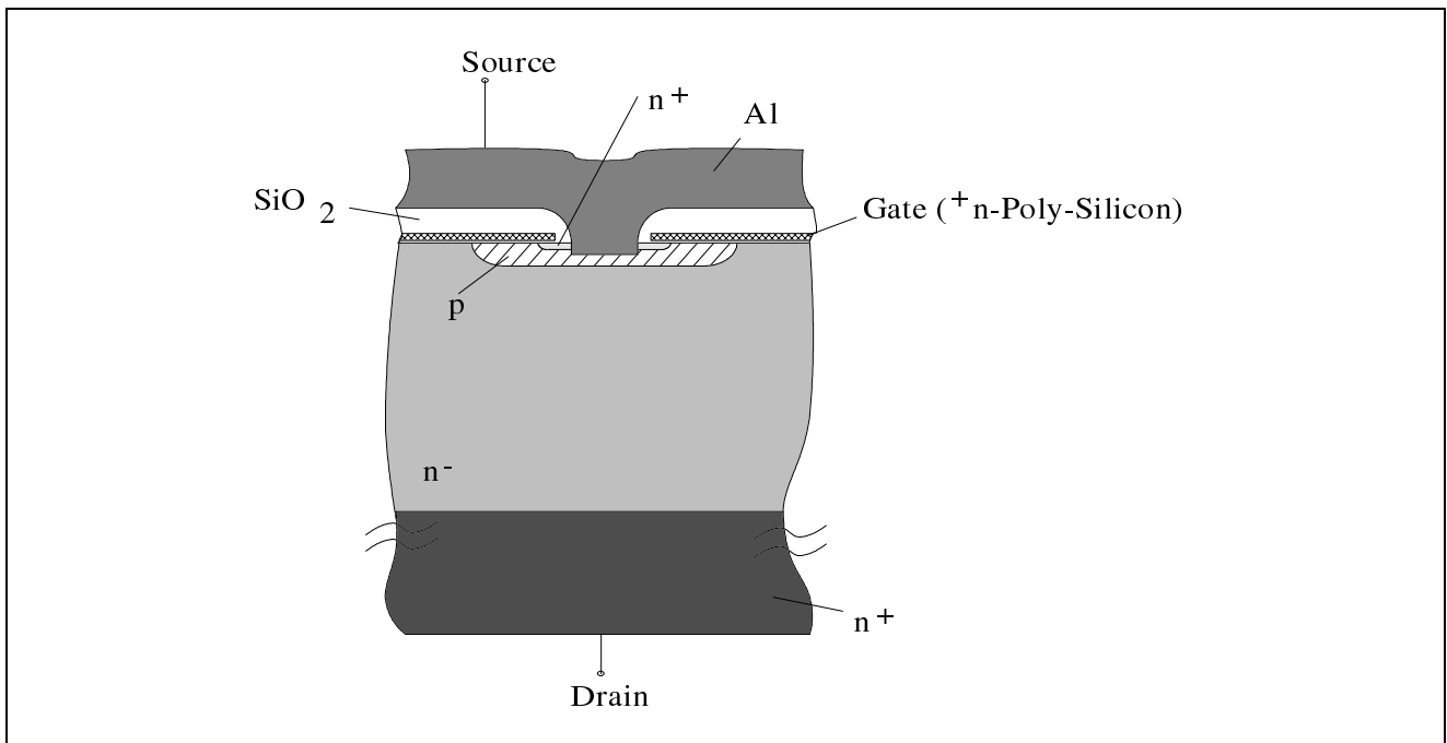
Figure 1 SIPMOS-Transistor (MOSFET)
