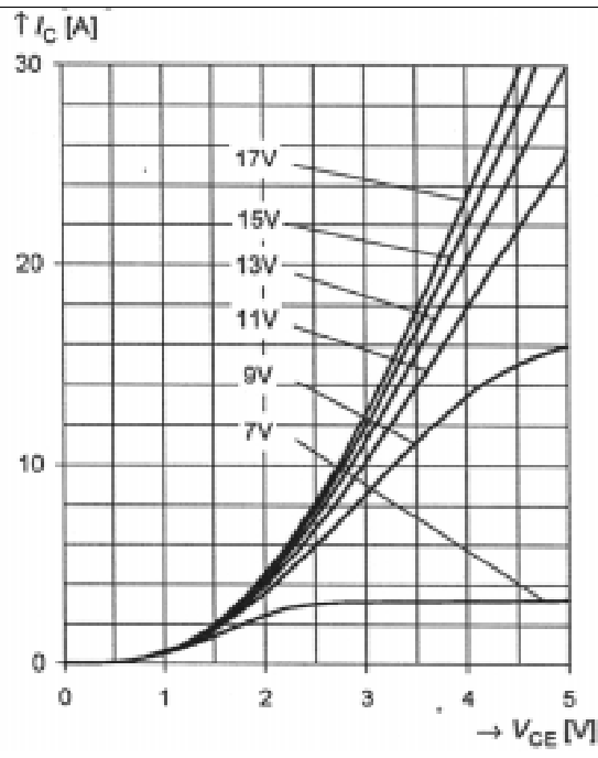
Figure 3 Output Characteristics of an IGBT BUP 314 (1000 V)
