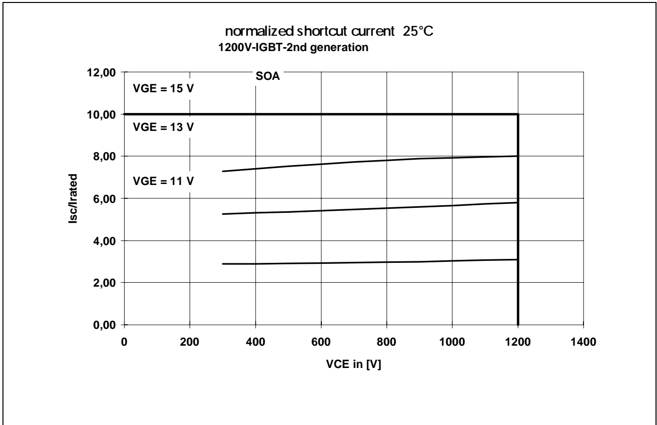
Figure 22 Safe Operating Area in Short-circuit Case
