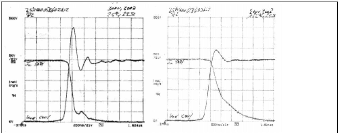
Figure 12 Strong Increase of Tail-Current With (left 25 °C, right 125 °C)
