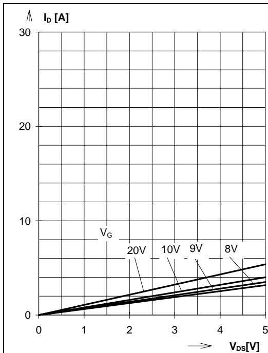
Figure 4 Output Characteristics of a MOSFET BUZ 312 (1000 V)
