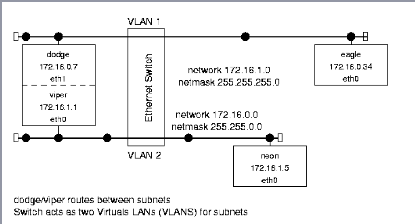
Figure 13.1: Experimental system setup.
