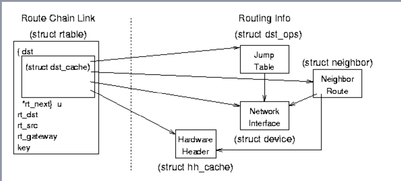
Figure 8.7: Destination Cache data structure relationships.
