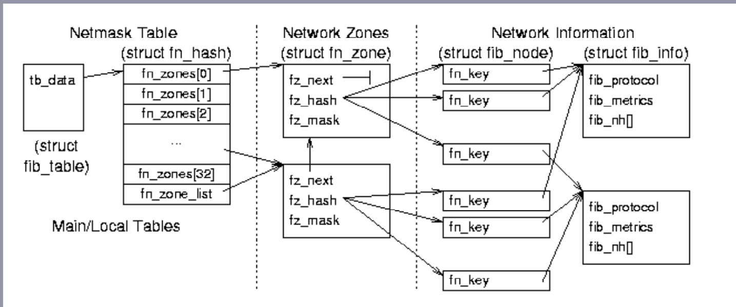
Figure 8.4: Forwarding Information Base (FIB) data relationships.
