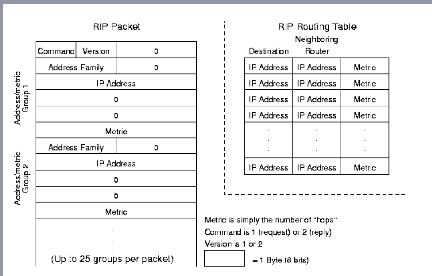
Figure 9.1: Routing Information Protocol packet and table.
