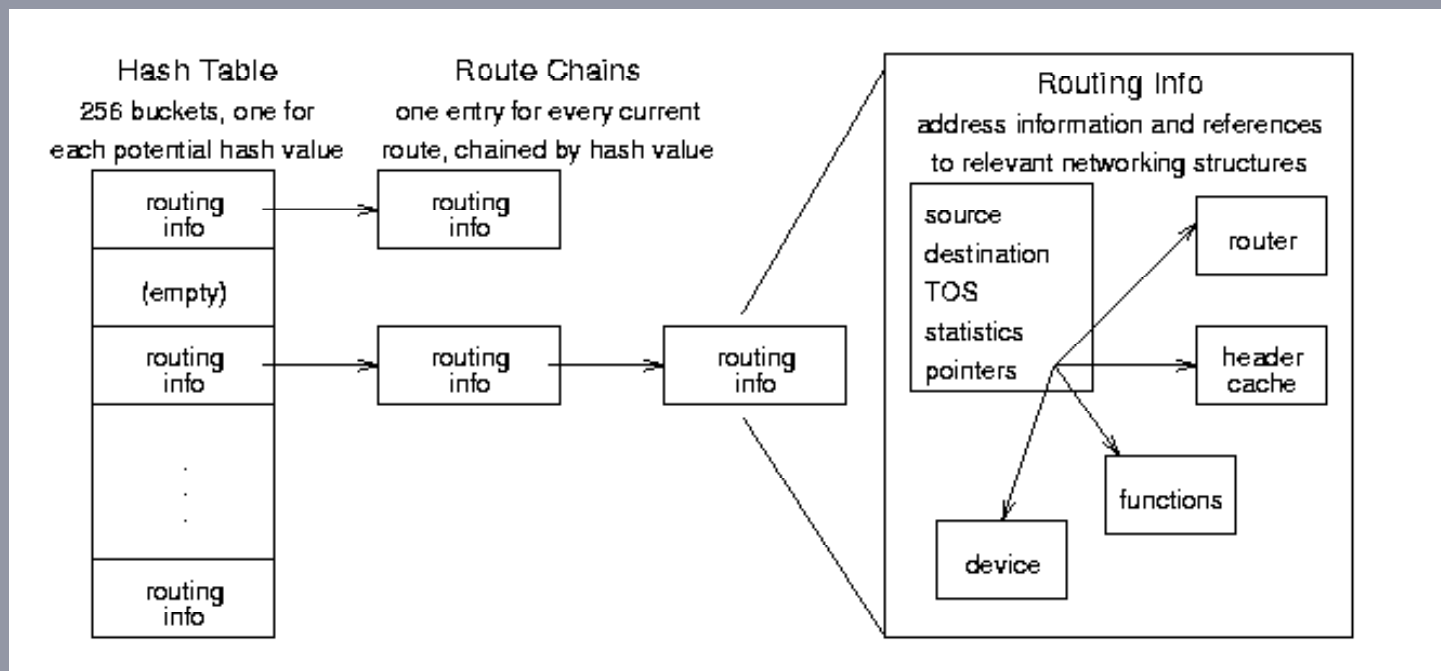
Figure 8.5: Routing Cache conceptual organization.
