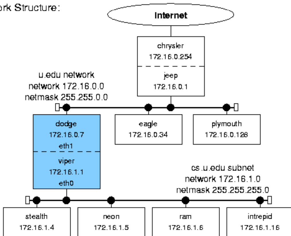
dodge/viper Routing Tables:
