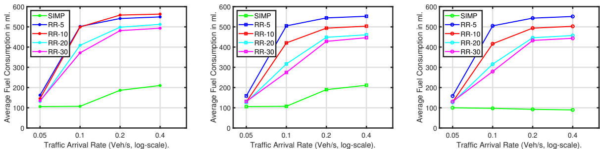
Fig. 3: Average Fuel Consumption results in \text{ml} for Scenarios-1, 2, and 3 with 30\text{Km/h} speed limit from left to right.
