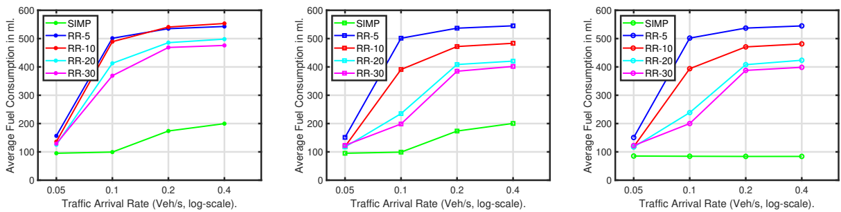
Fig. 5: Average Fuel Consumption results in ml, for Scenarios-1, 2, and 3 with 50Km/h speed limit from left to right accordingly.
