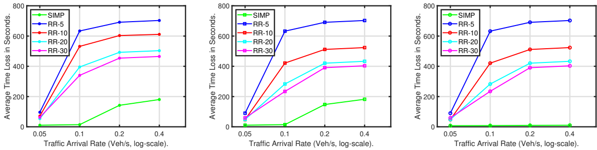
Fig. 2: Average Time Loss results in seconds, for Scenarios-1, 2, and 3 with 30\text{Km/h} speed limit from left to right.
