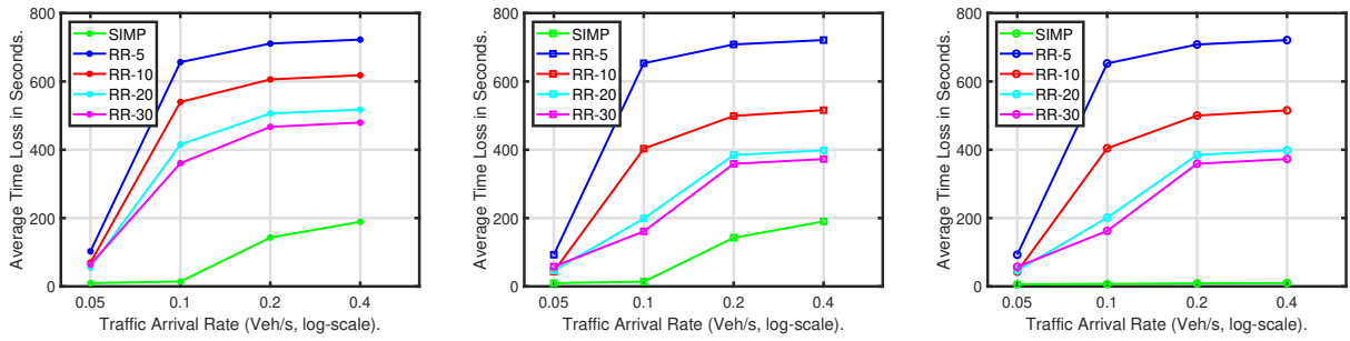
Fig. 4: Average Time Loss results in seconds, for Scenarios-1, 2, and 3 with 50Km/h speed limit from left to right.
